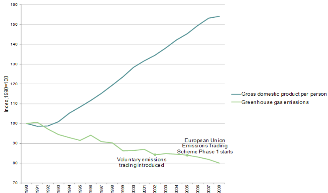
Figure 2. Economic growth coupled with reduced greenhouse gas emissions in the UK
